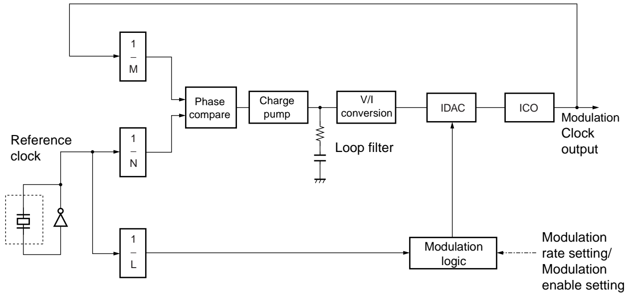
MB88154A PLL block
