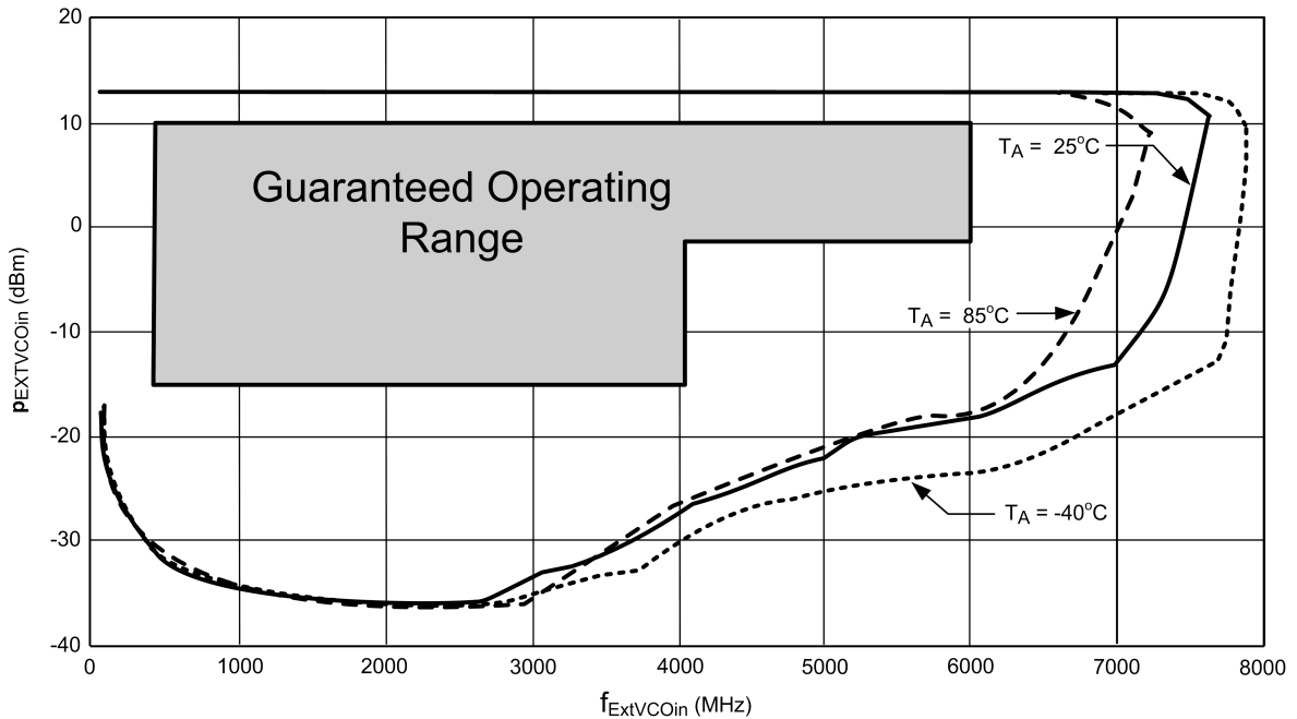
SINE wave ExtVCOin Sensitivity
