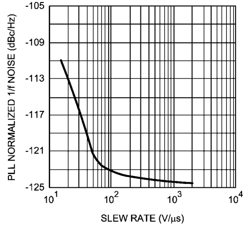
PLL Normalized 1/f Noise vs. OSCin Slew Rate ( K_{PD} = 32X )
