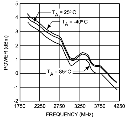
Output Power vs. Temperature (VCO_DIV = 1, VCOGAIN = 12, OUTTERM = 12, V_{CC} = 3.3\text{ V} (Note 6))
