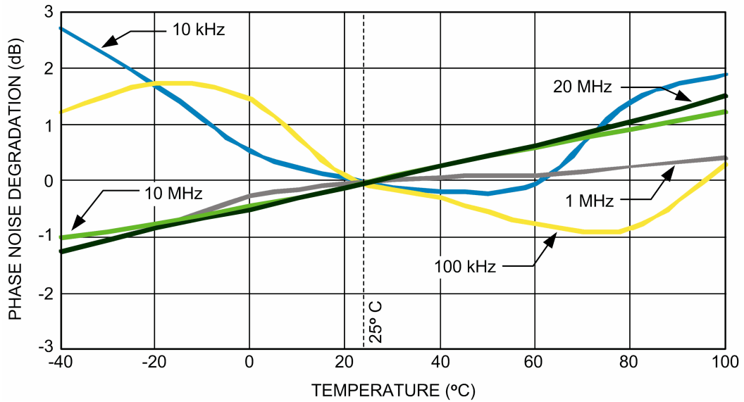
VCO Phase Noise Degradation vs. Temperature and Offset (VCO Relocked at Each Temperature V_{CC} = 3.3\text{ V} , AC\_TEMP\_COMP = 5 )
