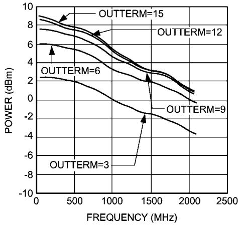
Output Power vs. OUTTERM and FREQUENCY (VCO_DIV > 1, T A = 25 °C, Vcc = 3.3 V, DIVGAIN = 12 (Note 6) )
