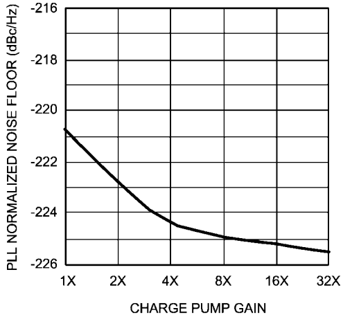
PLL Normalized Noise Floor vs. Charge Pump Gain (Slew Rate = 2000 V/μs)
