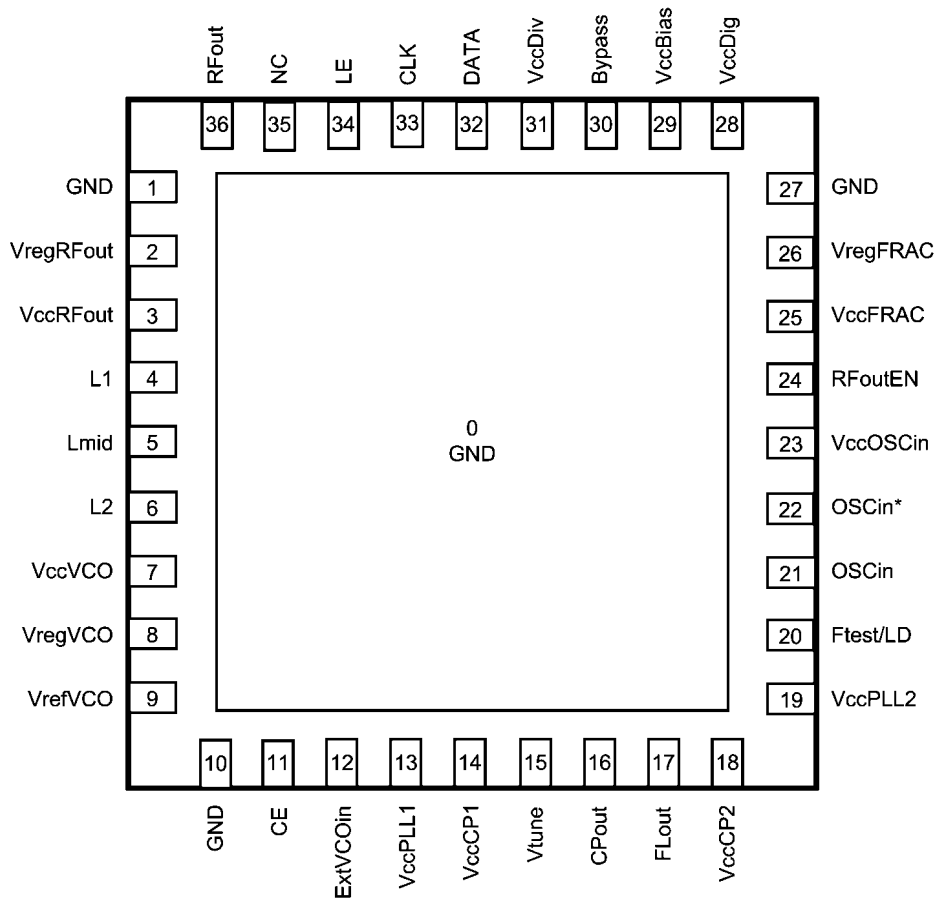
36-Pin SQ Package (Top View)
