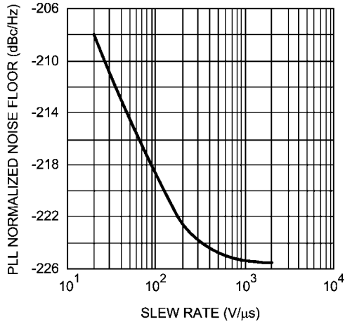
PLL Normalized Noise Floor vs. OSCin Slew Rate ( K_{PD} = 32X )
