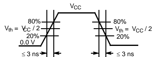
CMOS Input Test Waveform (CY7B9920)
