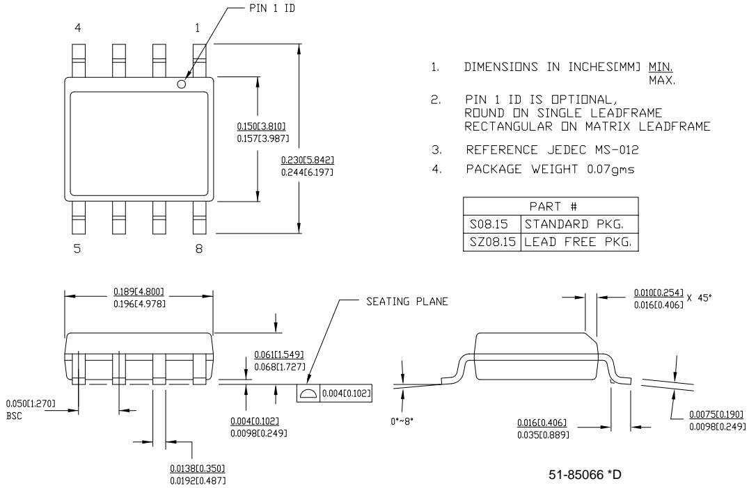
Figure 6. 8-Pin (150-Mil) SOIC S8
