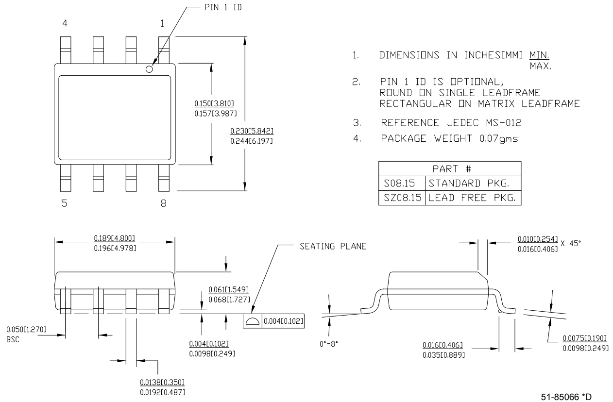
Figure 4. 8-Pin (150-Mil) SOIC S8
