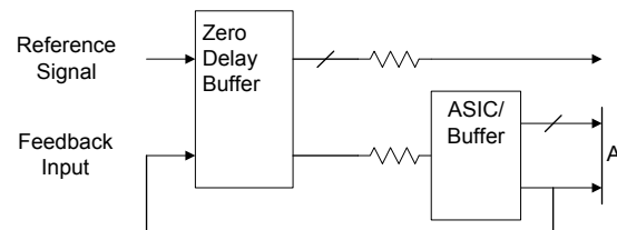
Figure 3. Six Output Buffer in the Feedback Path
