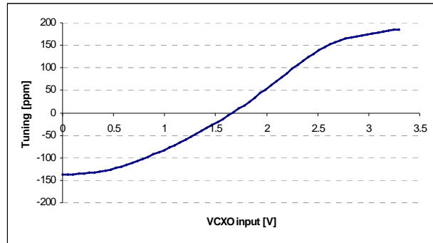
Figure 2. VCXO Profile
