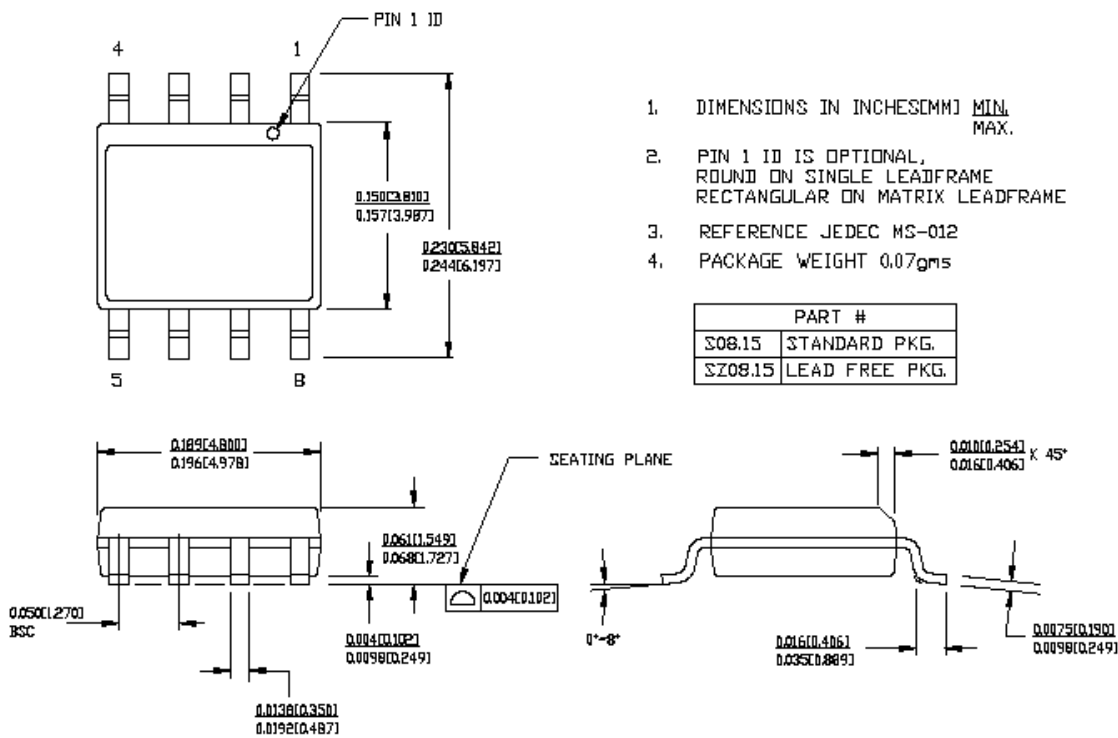
Figure 6. 8-Lead (150-Mil) SOIC S8
