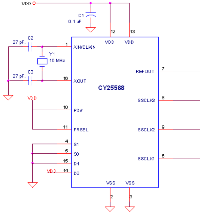
Figure 8. Application Schematic
