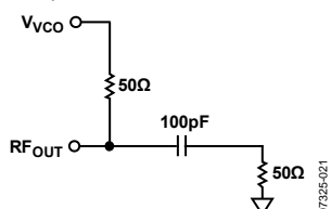
Figure 37. Simple ADF4350 Output Stage
