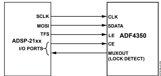
Figure 36. ADSP-21xx to ADF4350 Interface
