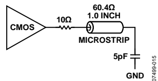
Figure 15. Series Termination of CMOS Output
