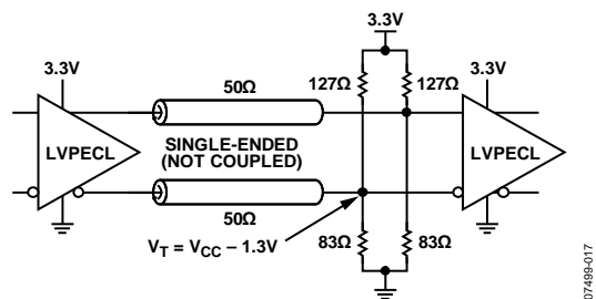
Figure 17. LVPECL Far-End Termination
