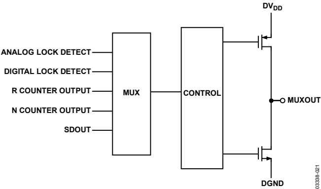
Figure 21. MUXOUT Circuit
