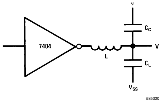
FIGURE 5. Clock Coupling
