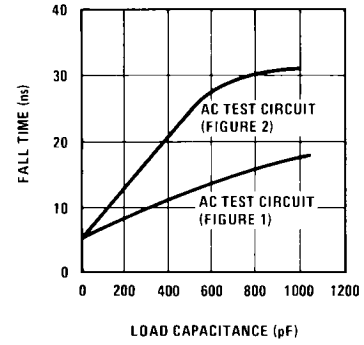
Fall Time vs Load Capacitance
