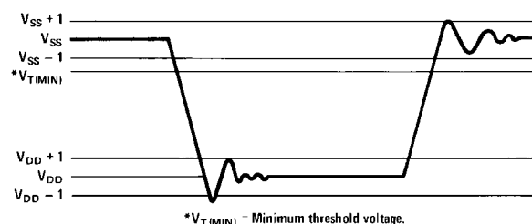
FIGURE 3. Clock Waveform
