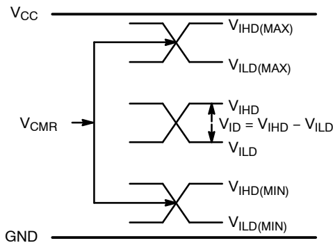
Figure 13. V_{CM} Diagram
