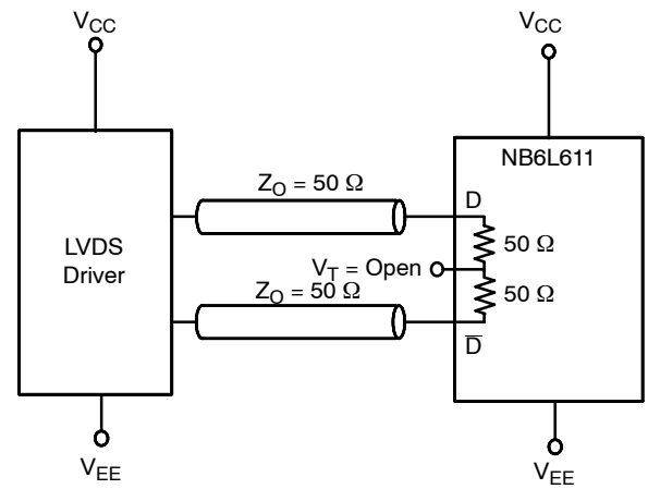
Figure 16. LVDS Interface
