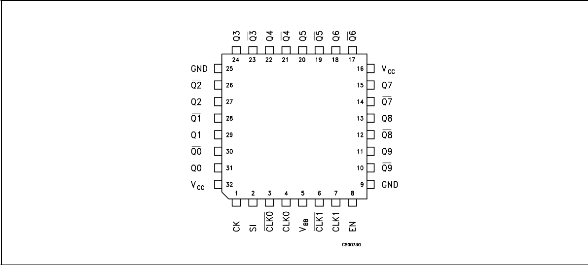
Figure 1. Pin connections
