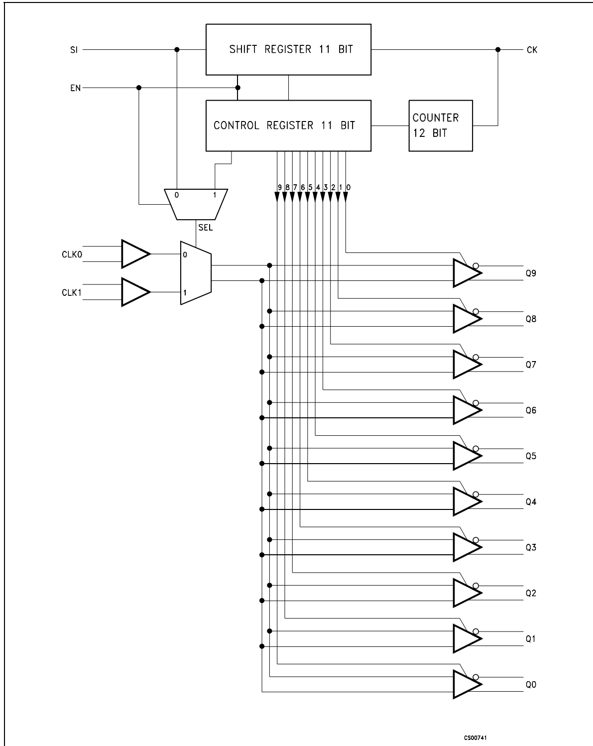
Figure 2. Logic diagram
