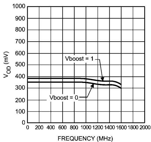
LVDS Differential Output Voltage ( V_{OD} )
