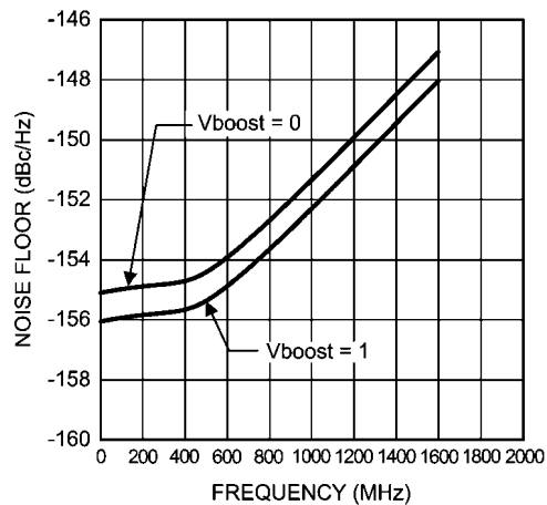
LVDS Output Noise Floor
