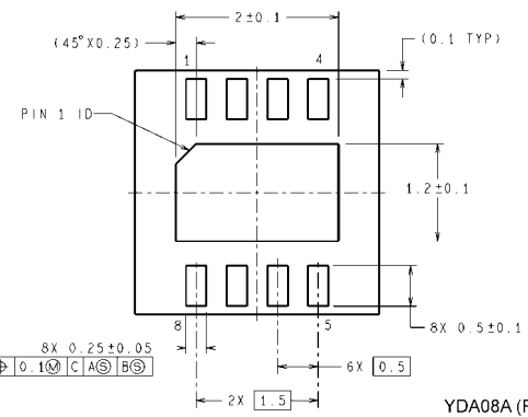
8-Pin LLP NS Package Number YDA08A
