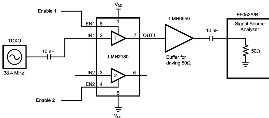
FIGURE 5. Measurement Setup
