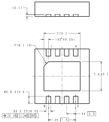
SDA08A (Rev A)
