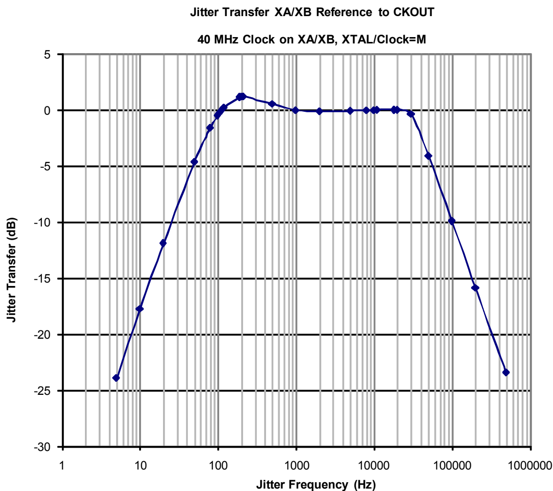
Figure 20. Typical XA/XB Reference Jitter Transfer Function
