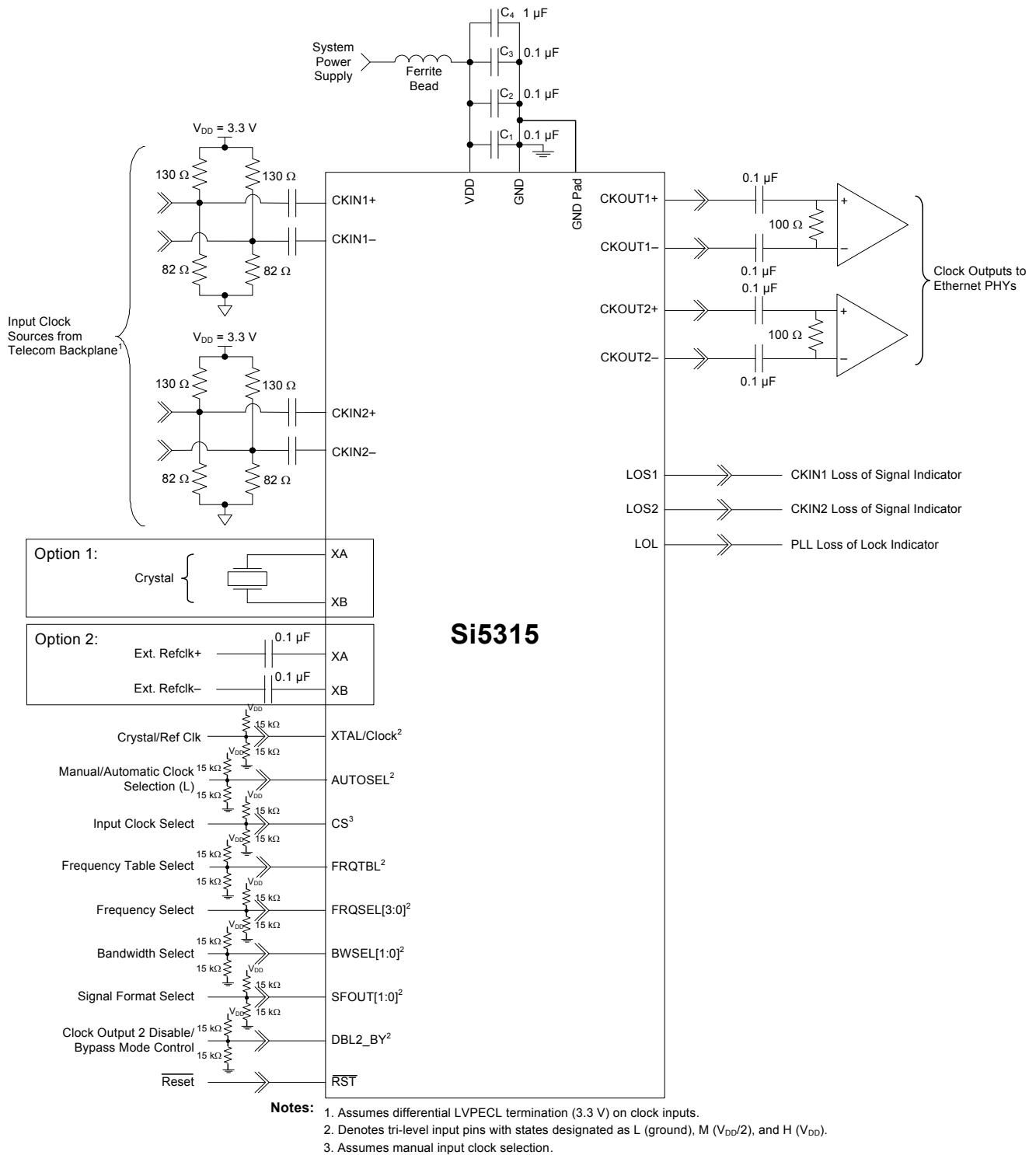
Figure 23. Si5315 Typical Application Circuit
