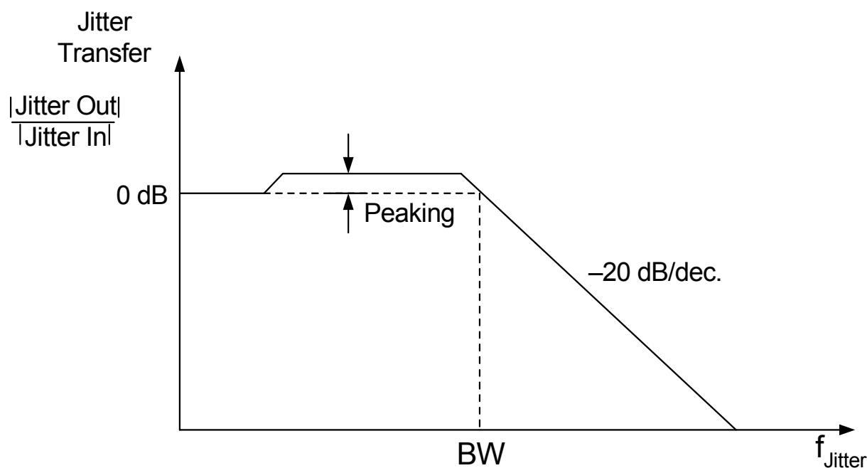
Figure 7. PLL Jitter Transfer Mask/Template
