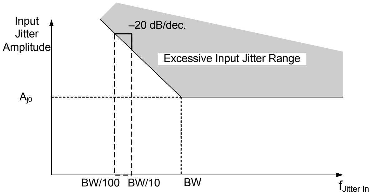
Figure 8. Jitter Tolerance Mask/Template
