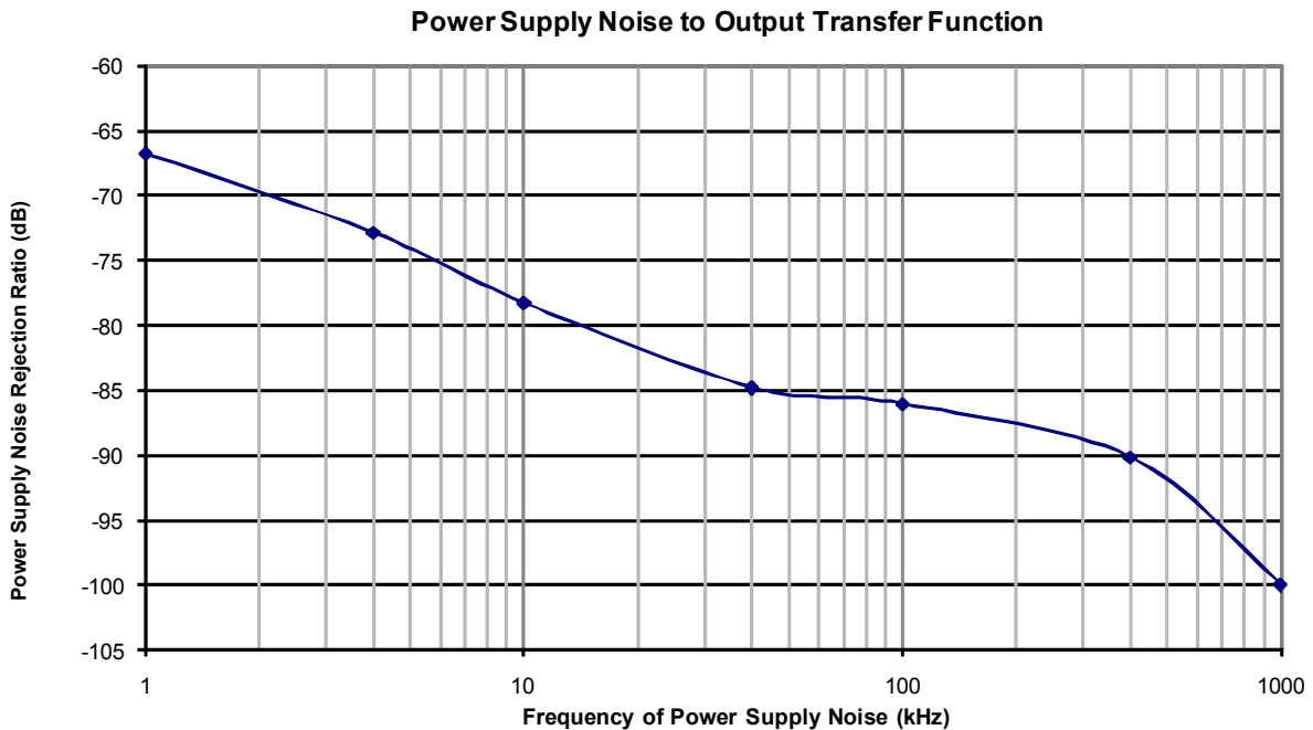
Figure 22. f_{out} = 155 MHz with 112 Hz Loop Bandwidth, 100 mVp-p Supply Noise
