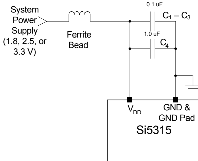
Figure 21. Typical Power Supply Bypass Network
