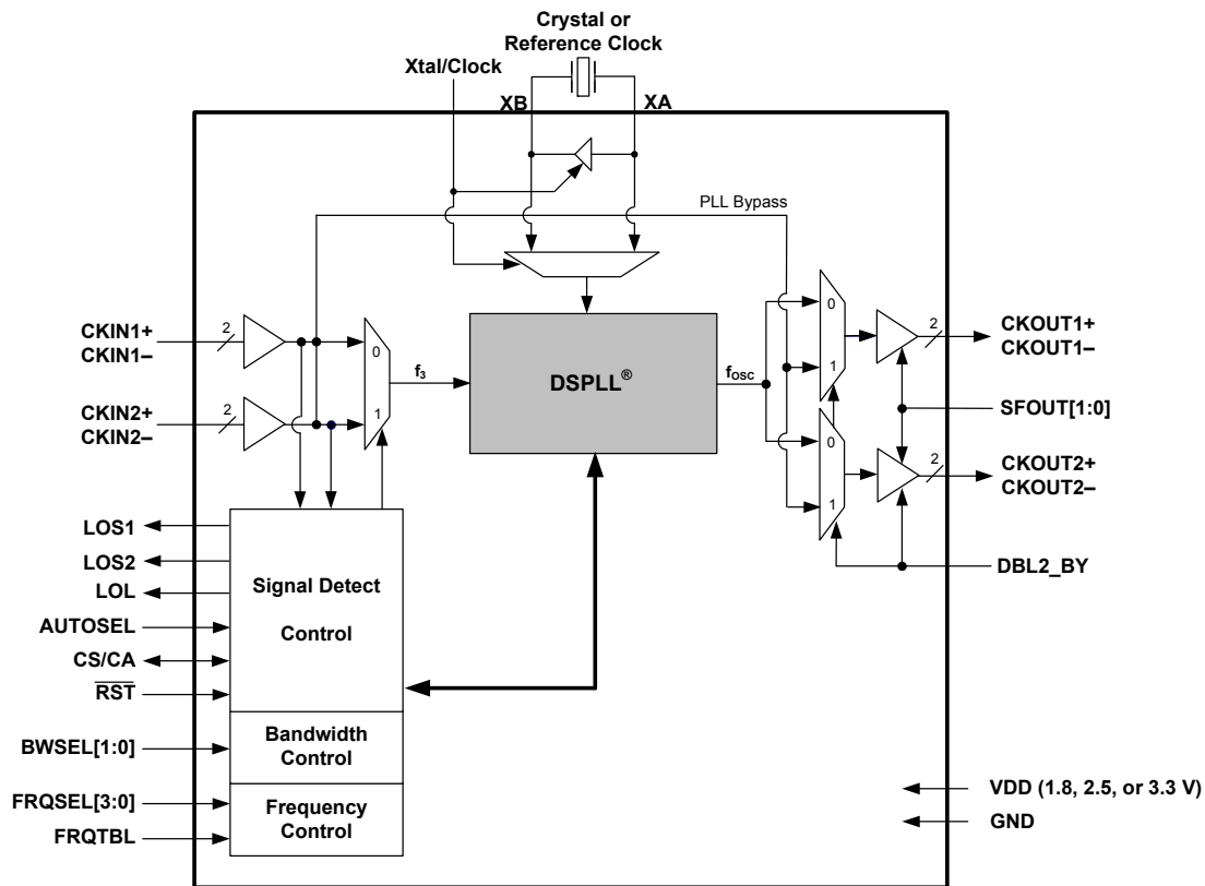
Figure 6. Detailed Block Diagram
