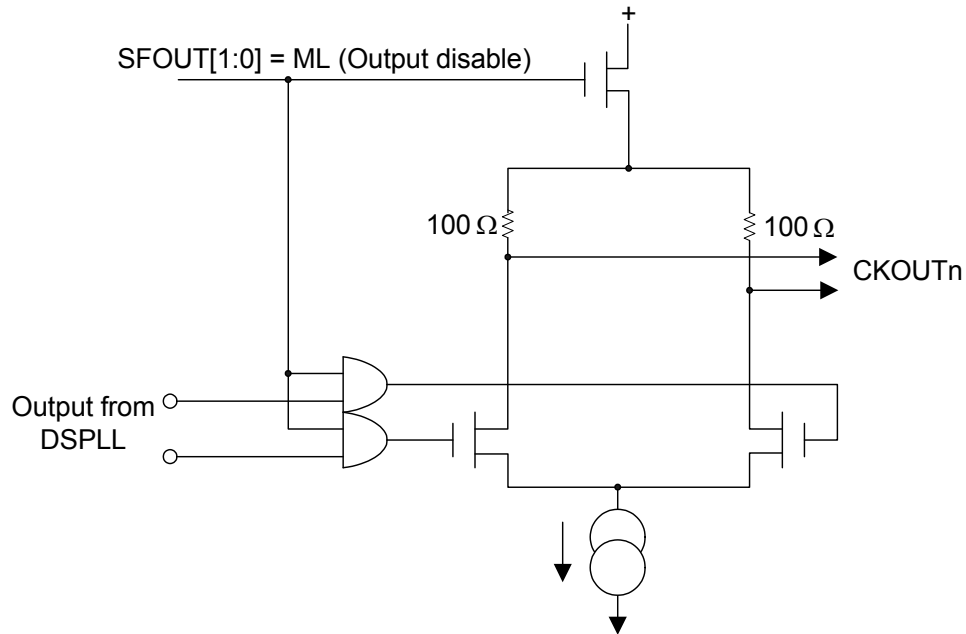
Figure 16. Disable CKOUTn Structure
