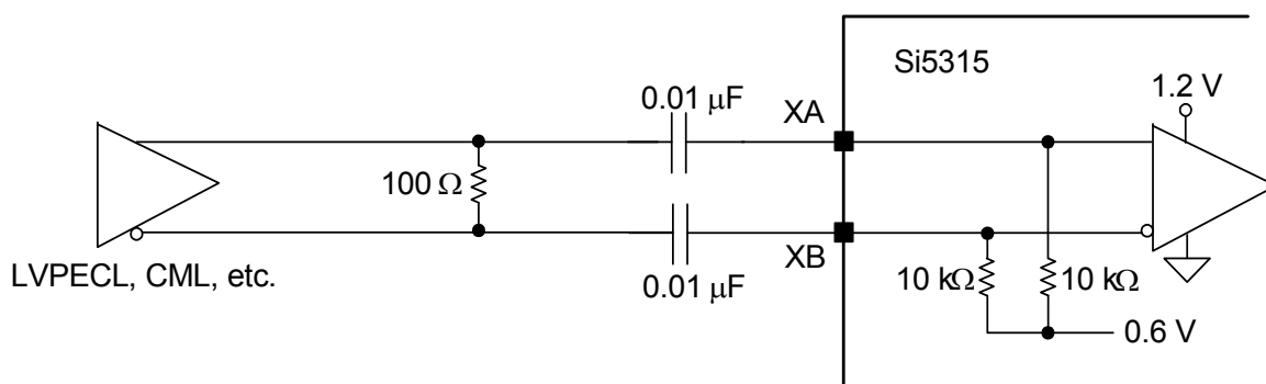
Figure 19. Differential External Reference Clock Input Example
