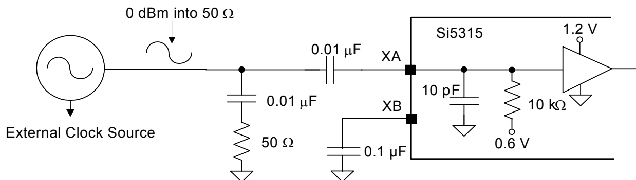
Figure 18. Sinewave External Reference Clock Input Example
