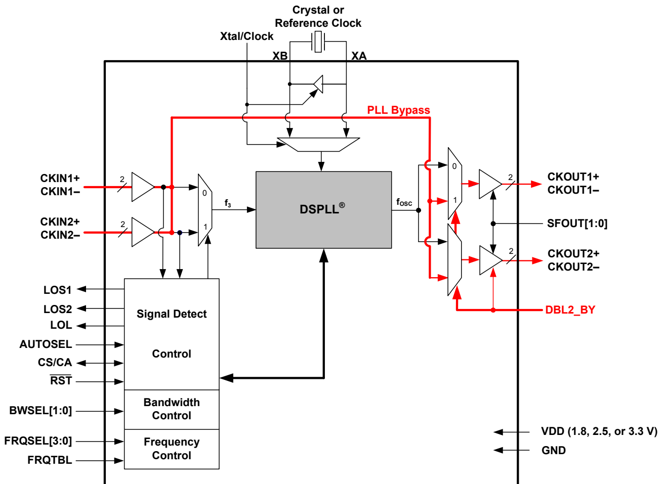
Figure 9. Bypass Signal
