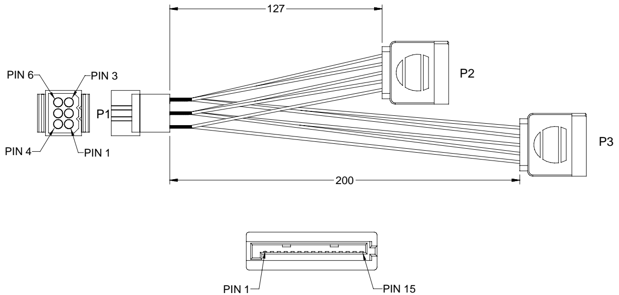
SATA 15 Position Plug Ends Typ. for P2 and P3
