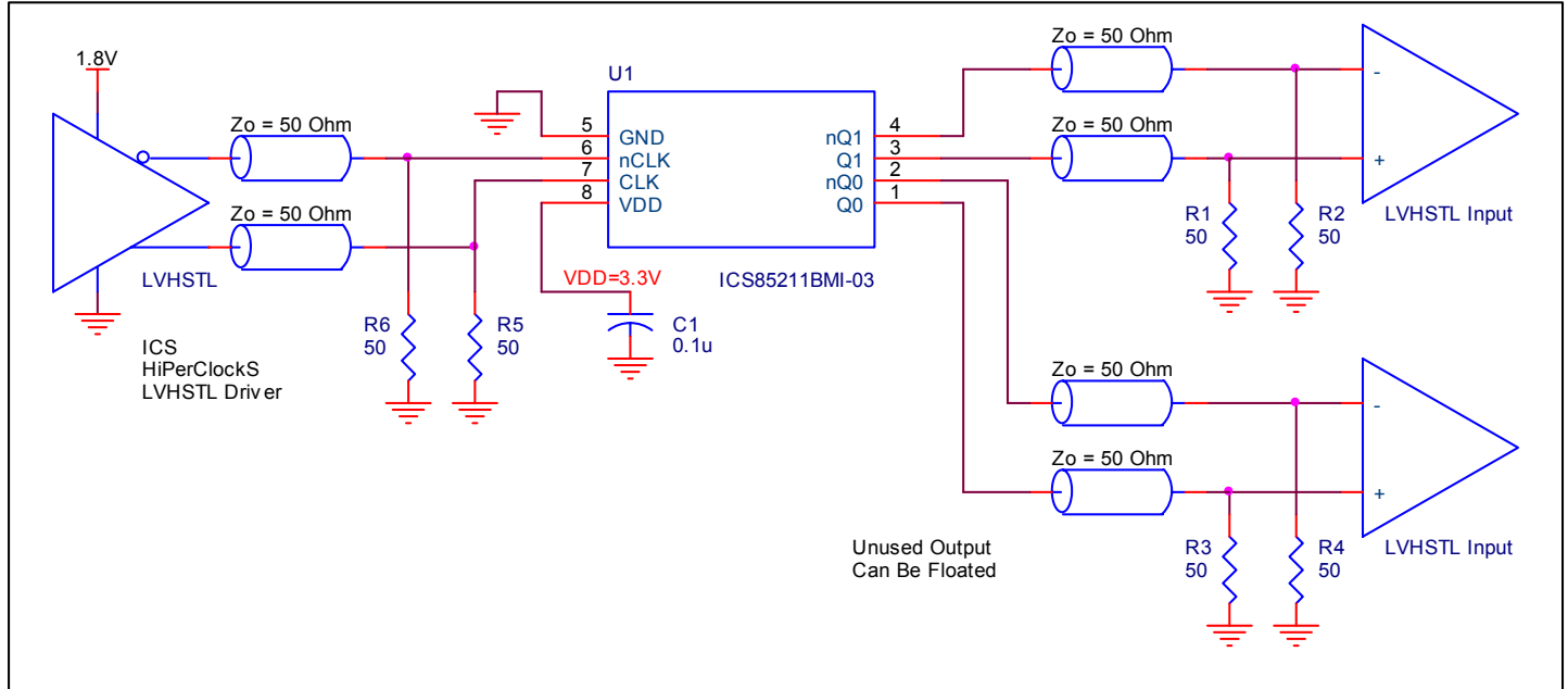
Figure 3. ICS85211BI-03 LVHSTL Buffer Schematic Example
