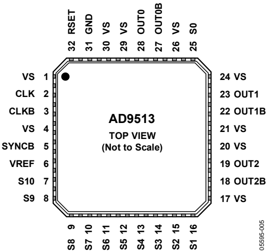
Figure 5. 32-Lead LFCSP Pin Configuration
