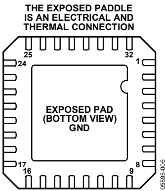
Figure 6. Exposed Paddle
