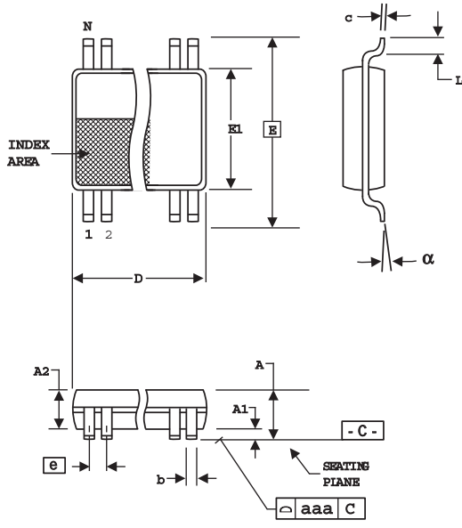
6.10 mm. Body, 0.50 mm. pitch TSSOP (240 mil) (0.020 mil)
