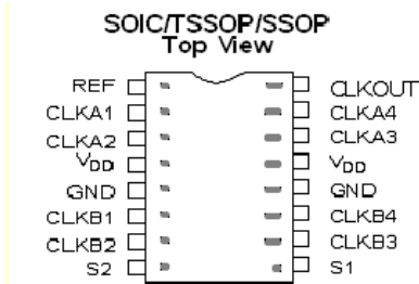
Figure 1. Pin Configuration – CY23S09
