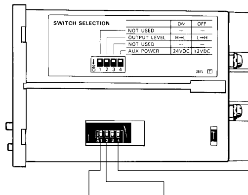
Dip switch
