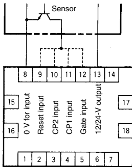
*H: Transistor ON
