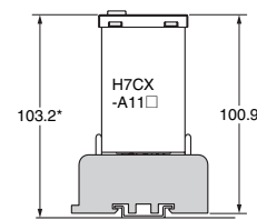
P2CF-11(-E) Front Connecting Socket (order separately)
