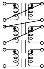
Figure 7 Turns ratio: 4:1:1
