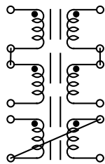
Figure 2 Turns ratio: 1:1:1
