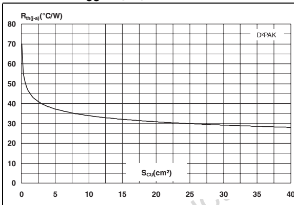
Figure 11. Variation of thermal resistance, junction to ambient versus copper surface area under tab (PCB FR4, e CU 35 μm)
