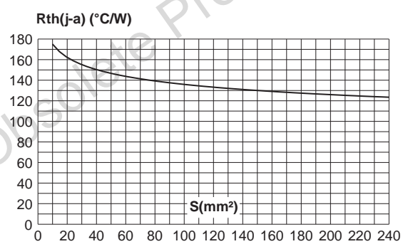
Fig. 13: Thermal resistance junction to ambient versus copper surface under tab (Epoxy printed circuit board FR4, copper thickness under "com" pins: 35\mu\text{m} ) (ACS102-5T1).
