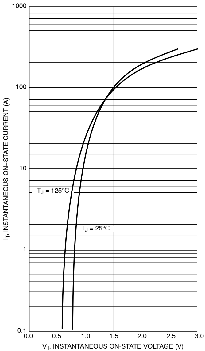
Figure 3. On-State Characteristics
