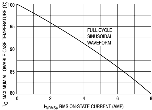
Figure 1. Current Derating
