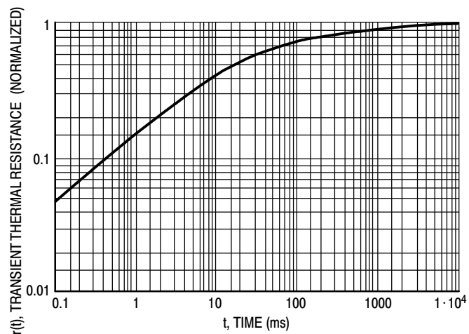
Figure 4. Thermal Response
