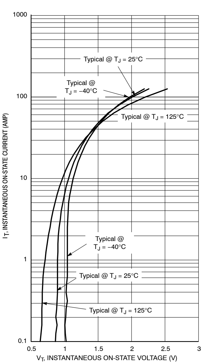
Figure 3. On-State Characteristics
