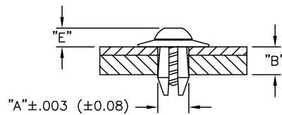
TYPICAL ASSEMBLY
