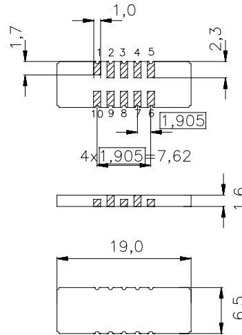
Ceramic package DCC18
