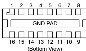
Figure 3. Pin Diagram
