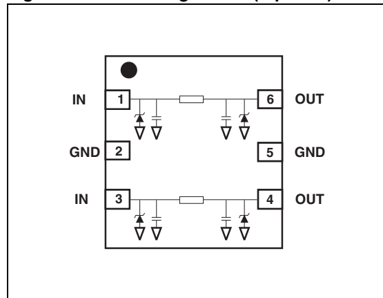
Figure 2. Basic cell configuration
