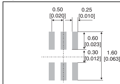
Figure 10. Footprint in mm [inches]
