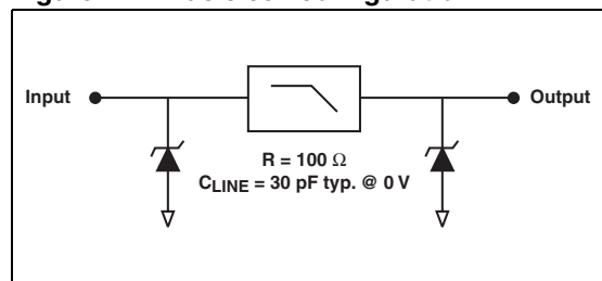
Figure 2. Basic cell configuration
