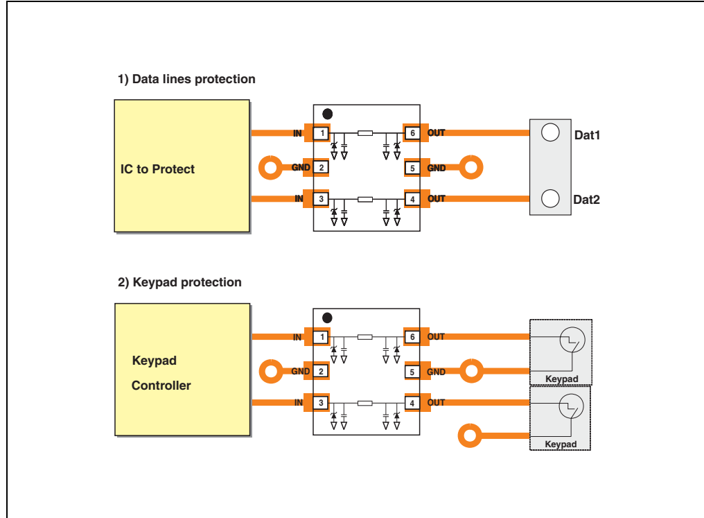
Figure 8. Application schematic
