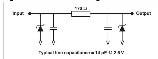
Figure 2. Basic cell configuration
