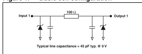
Figure 1. Basic cell configuration
