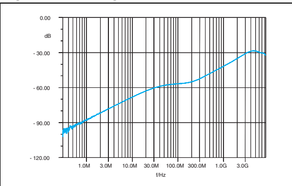
Figure 4. Analog cross talk measurements
