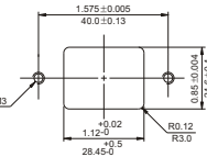
SUGGESTED MOUNTING CUTOUT
