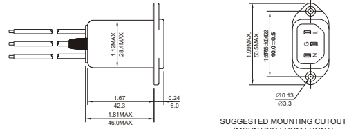
SUGGESTED MOUNTING CUTOUT (MOUNTING FROM FRONT)
