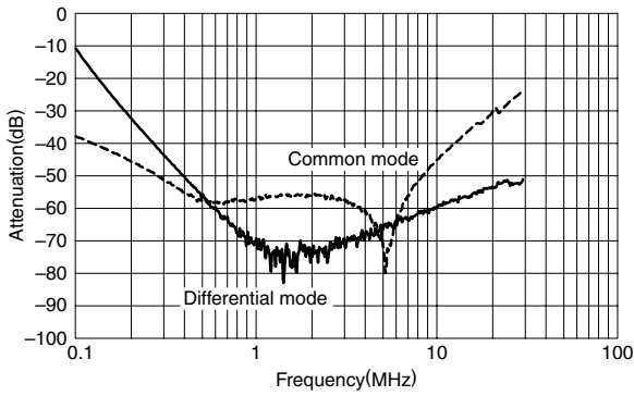
RSEL-20R5W/A
