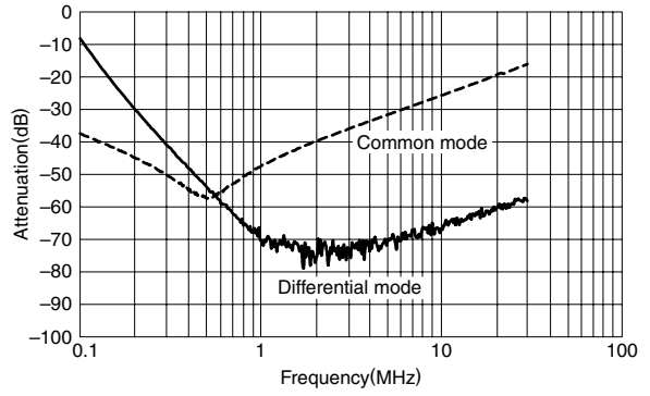
RSEL-2001WL/AL
