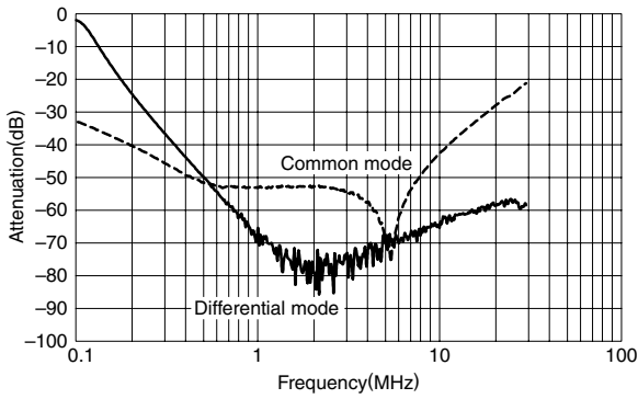
RSEL-2002W/A
