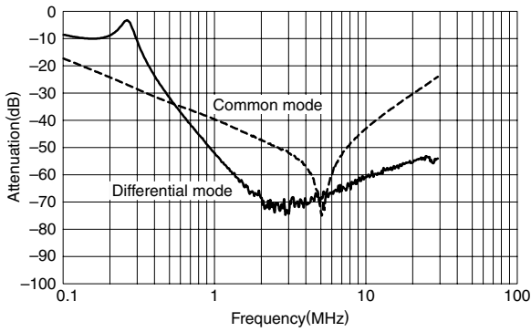
RSEL-2006W/A
