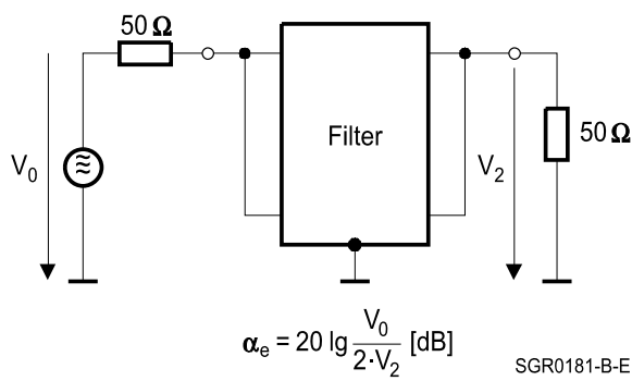
Asymmetrical measurement to MIL-STD-220A
