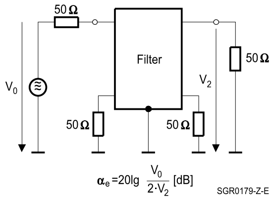
Unsymmetrical measurement circuit
