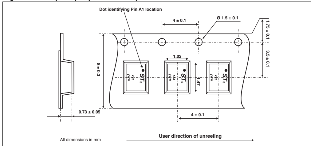
Figure 15. Flip Chip tape and reel specification
