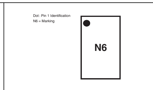
Figure 14. Marking
