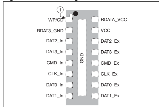
Figure 1. Pin configuration
