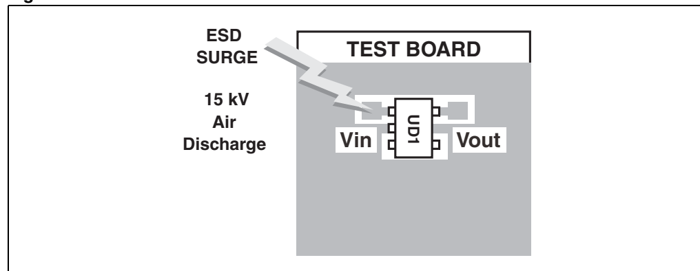
Figure 6. Measurement board
