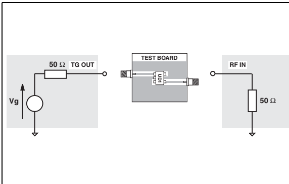
Figure 9. Analog crosstalk measurements
