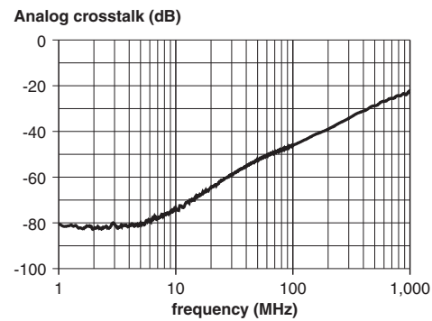
Figure 10. Typical analog crosstalk results
