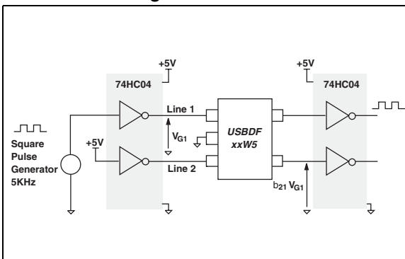
Figure 11. Digital crosstalk measurements configuration
