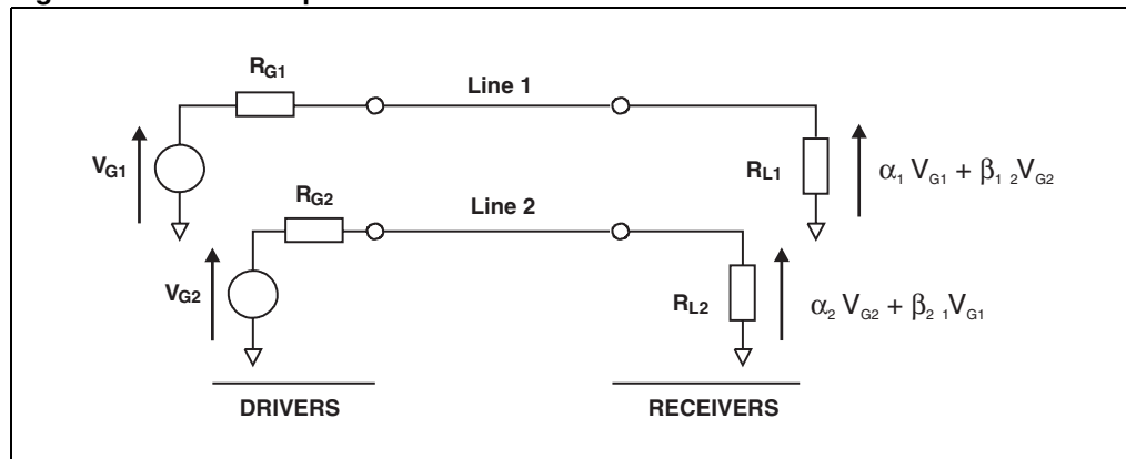
Figure 8. Crosstalk phenomena
