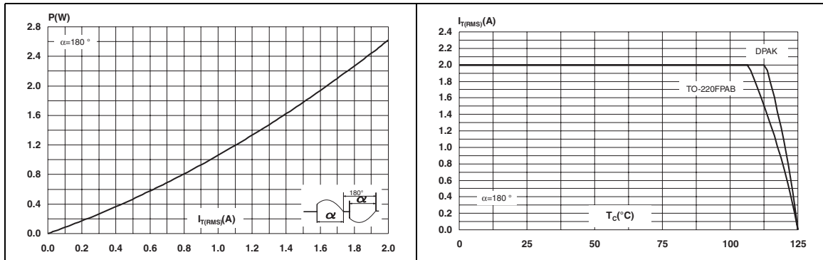
Figure 2. Maximum power dissipation versus on-state rms current (full cycle) Figure 3. On-state rms current versus case temperature
