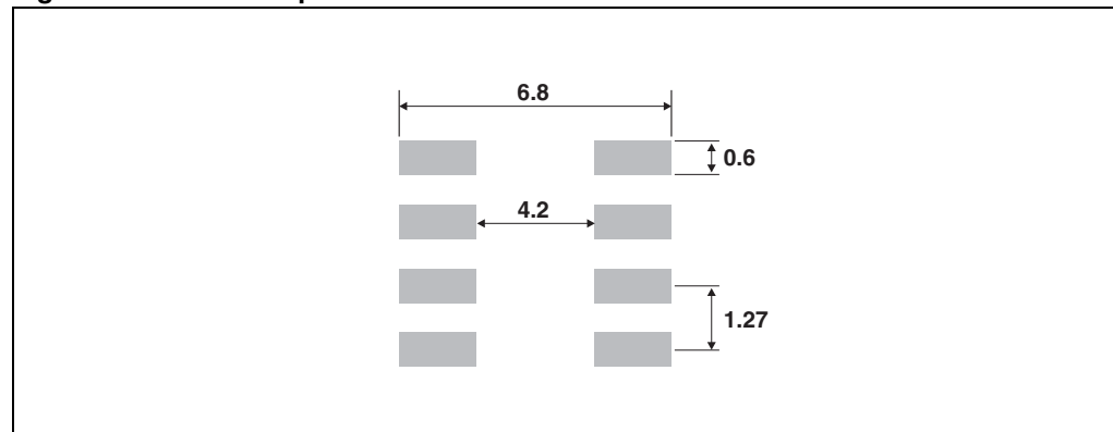
Figure 18. SO-8 Footprint
