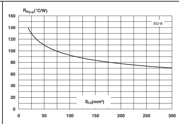
Figure 8. SO-8 junction to ambient thermal resistance versus copper surface under tab (PCB FR4, copper thickness 35 μm)
