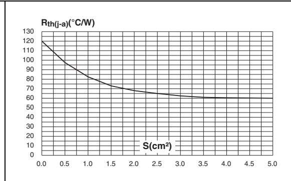
Figure 8. SOT-223 Thermal resistance junction to ambient versus copper surface under tab (printed circuit board FR4, copper thickness: 35 μm)
