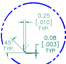
DETAIL "A" CHAMFER SCALE=5:1
