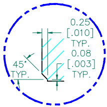
DETAIL "A" CHAMFER SCALE=8:1
