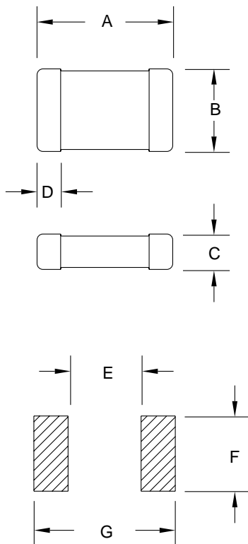
Pad Layout
