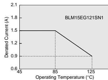
Derating
