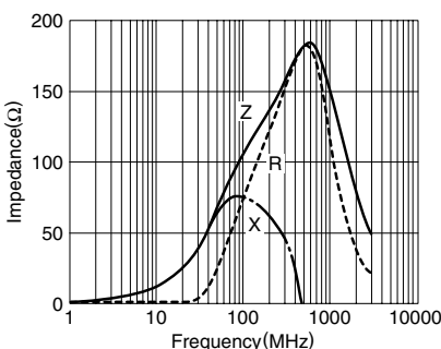
MPZ1608Y101B
