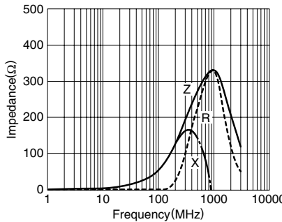
MPZ1608D600B
