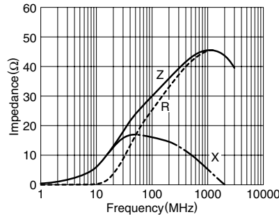
MPZ1005Y900C
