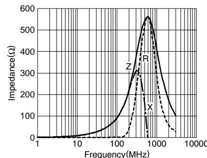
MPZ1608D101B
